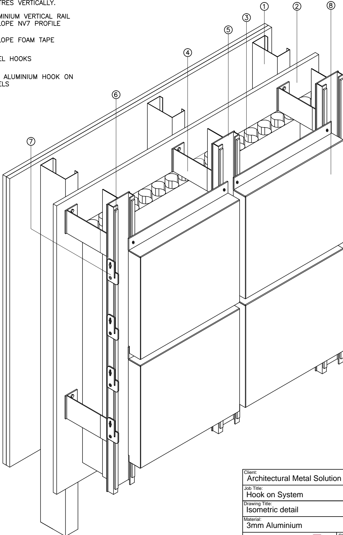
AMS-01 HOOK ON SYSTEM
